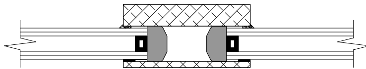
Mullion Cross-Section
